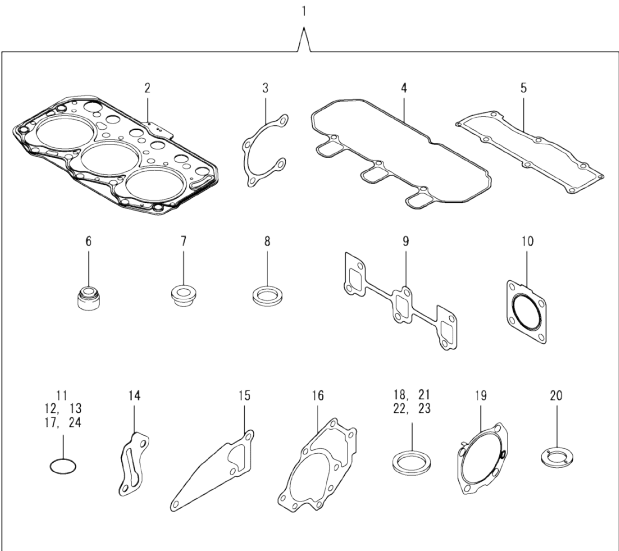
Fig.20. GASKET SET
